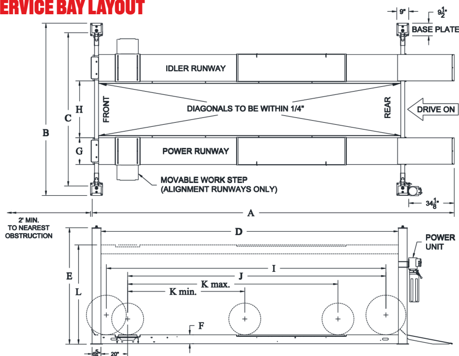
Fig 1 – General Specifications and Service Bay Layout
